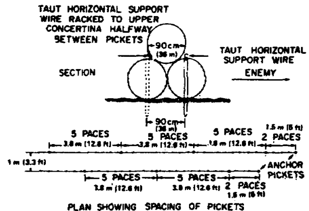
Figure 4-23. Triple standard concertina fence.
